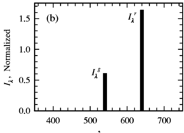
Fig. 5. Spectral irradiances for two lights that produce the same response for the average observer, a metameric match. (a) Monochromatic yellow light, \lambda^y = 580 nm. (b) The combination of monochromatic red and green lights, \lambda^r = 640 nm and \lambda^g = 540 nm.
